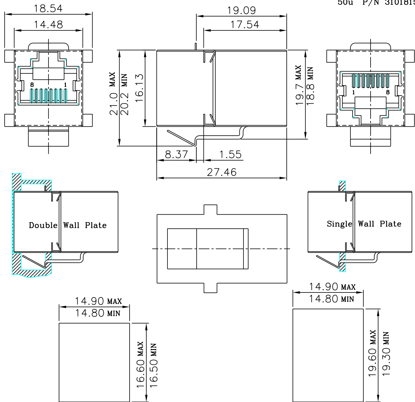
Front Panel Jack Only Clearance W/O Latch Feature
